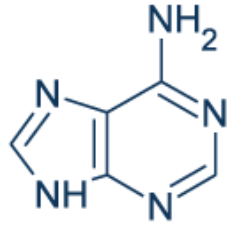
Adenine
